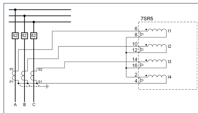
[dw_7SR5_ct-connection_diagram_01_2_en_US]
