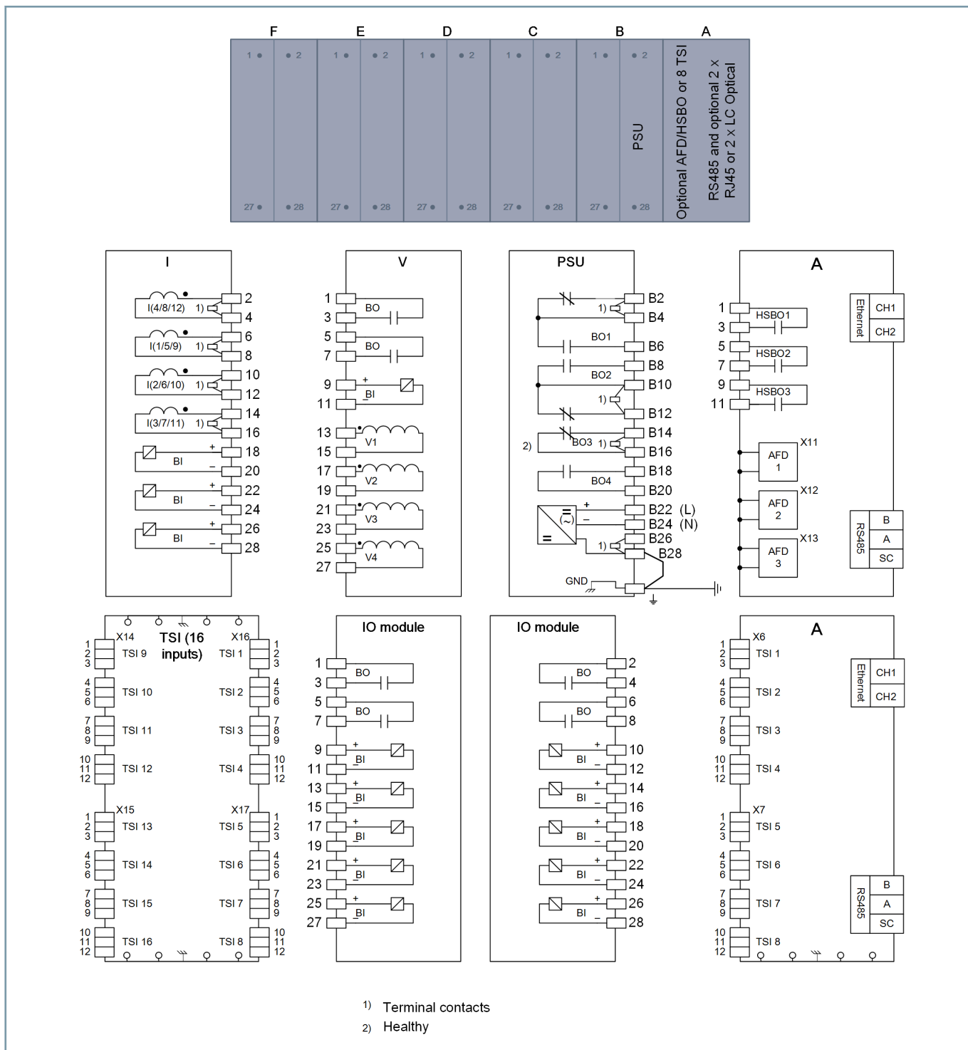
Figure 3.5/5 Rear View: Arrangement of Terminals and Modules
