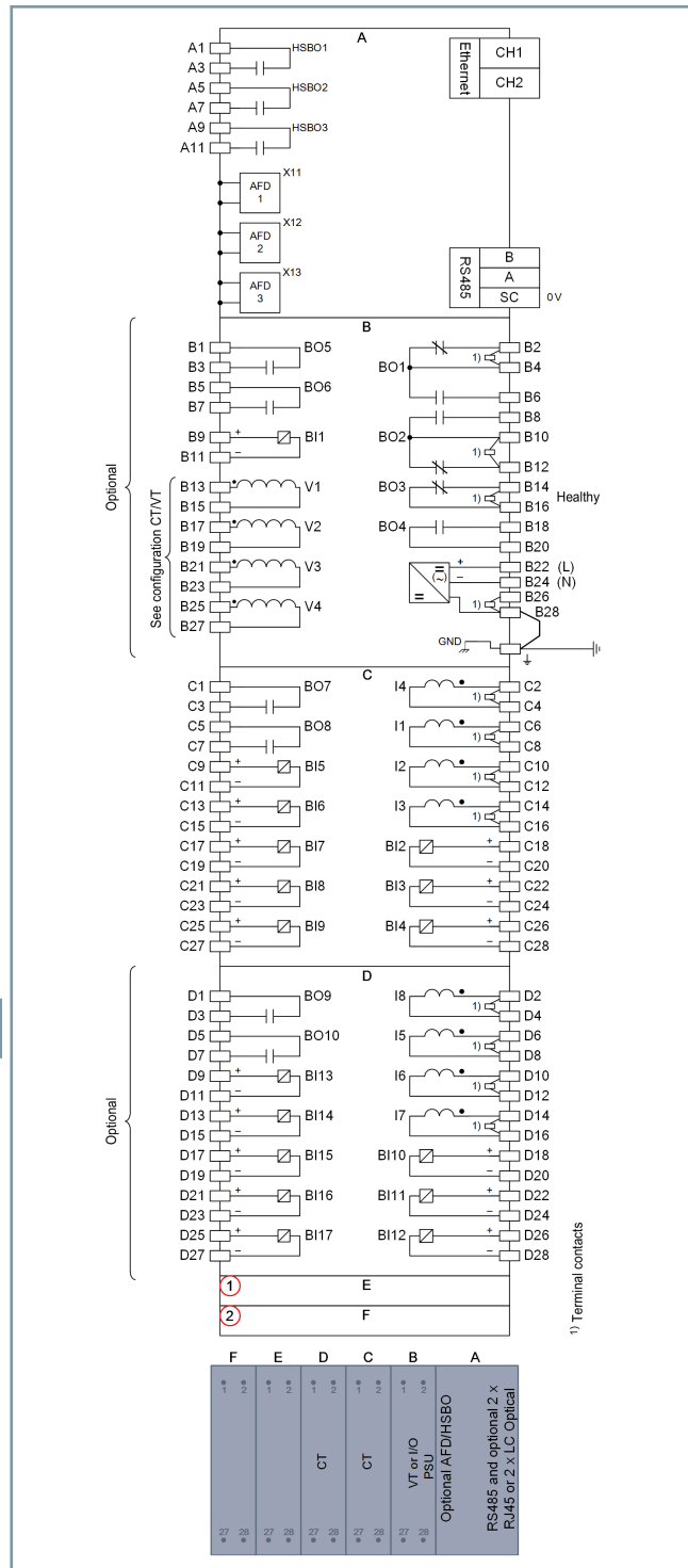
[HW_7SR5_transformer_wiring_diagram_8_en_US]
