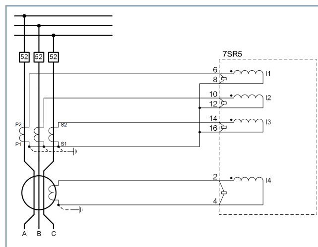
[dw_7SR5_ct-connection_diagram_02_3_en_US]
