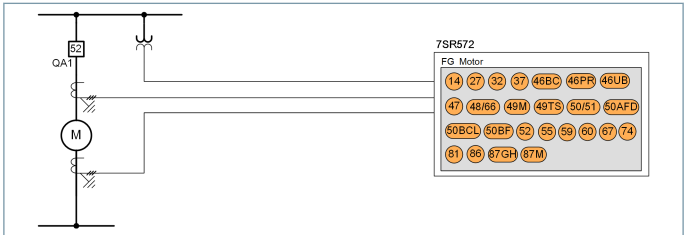
Figure 2.3/5 Motor: Differential Protection and Control
