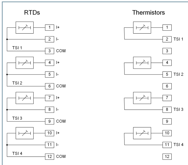
Figure 3.5/6 RTD or Thermistor Connections (Shown for Temperature Sensor Inputs (TSI) 1 to 4)
