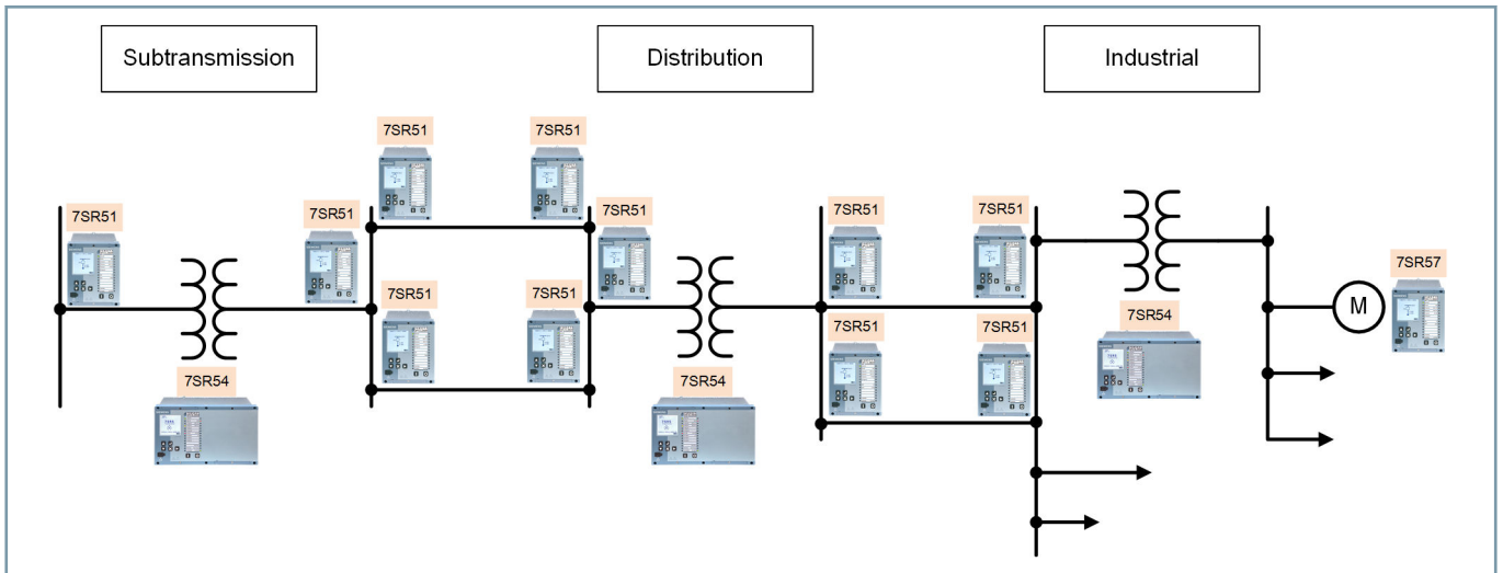
[dw_7SR5_devicetypes, 4, en_US]
